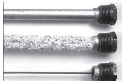
Figure 27 - Anode Rods from new (top) to partially depleted (middle) to fully depleted stage (bottom)
